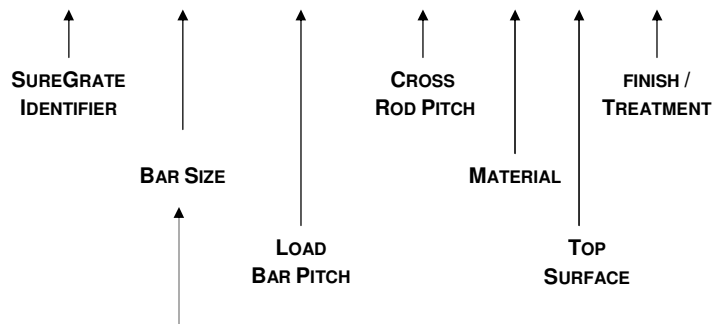
SG *** / 40 / 50 *** 40mm Load Bar Pitch 50mm Twist Bar Pitch
